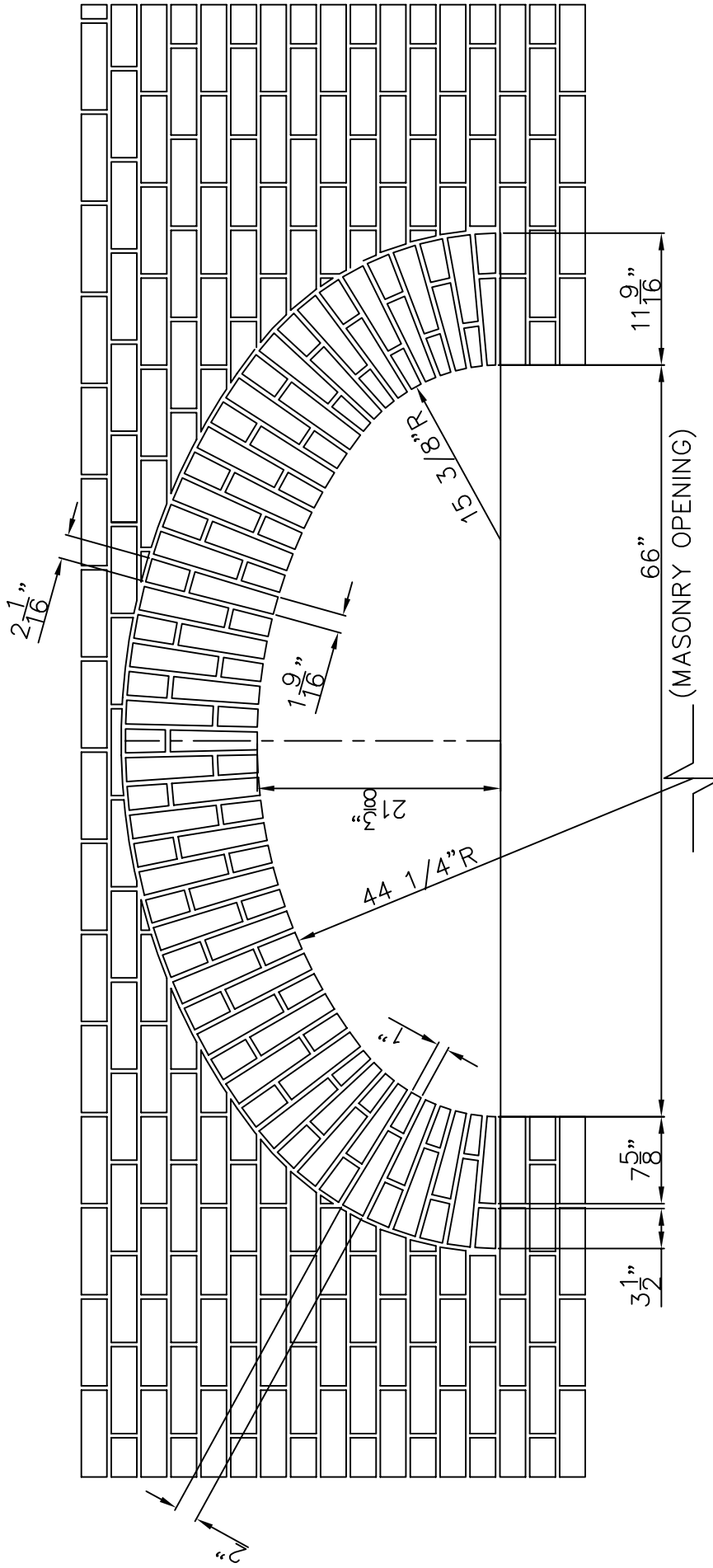
ELLIPTICAL ARCH C WITH BACKGROUND BRICK BRICK SIZE: MODULAR (6) REQ'D @ 98 PCS. EA.
