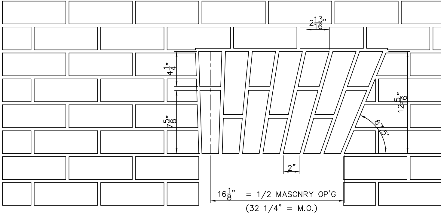
JACKARCH A BRICK SIZE: ENGINEER MODULAR (1) REQ'D @ 26 PCS. EA.
