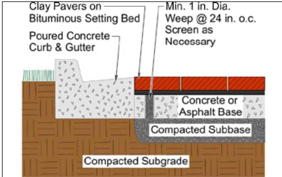
Paving - Poured Concrete Curb & Gutter Edge Restraint
