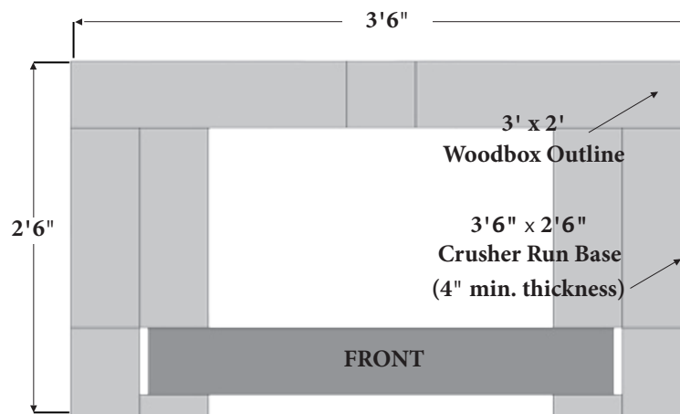
(Base Plan View)
