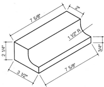
205-Cove Stretcher
