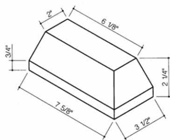
306-Outside Return Left
