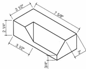
302-Splay Inside Return Right
