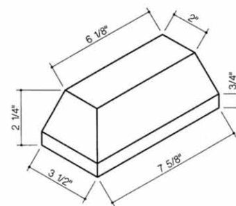
307-Outside Return Right
