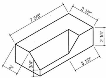
301-Splay Inside Return Left
