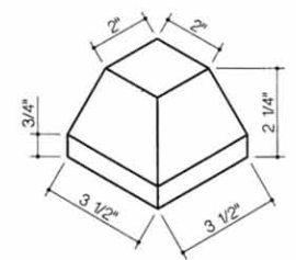
304-Splay Outside Corner
